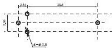
接线图 (底视图) Wiring diagram (Bottom view)
